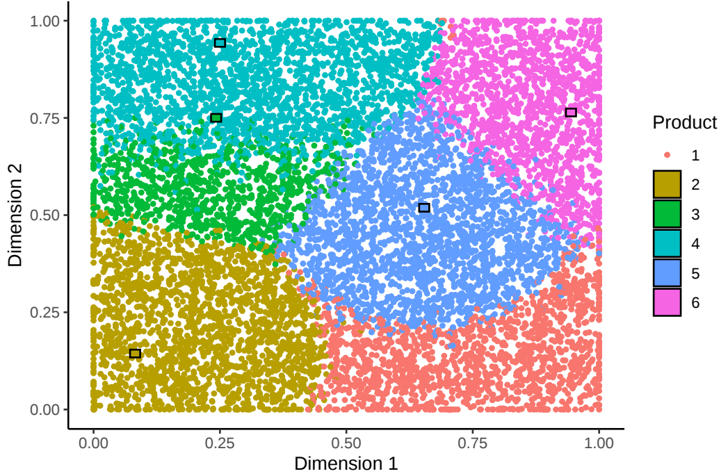
Figure A42: Simulated choice regions
