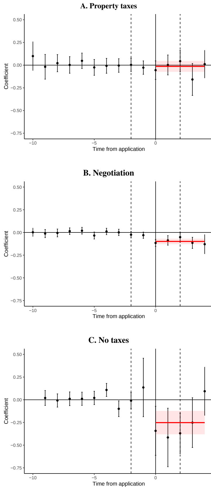
Figure A24: Price effects by tax regime
