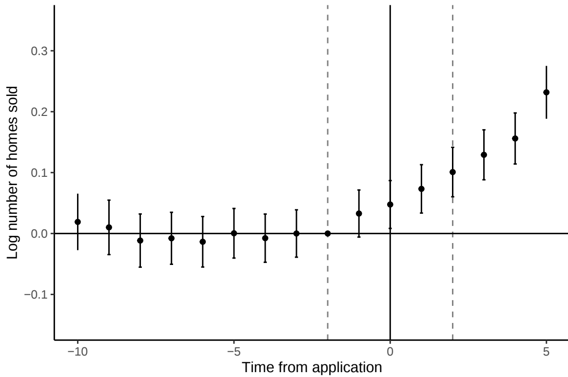
Figure A6: Effects of wind farm entry on home sales
