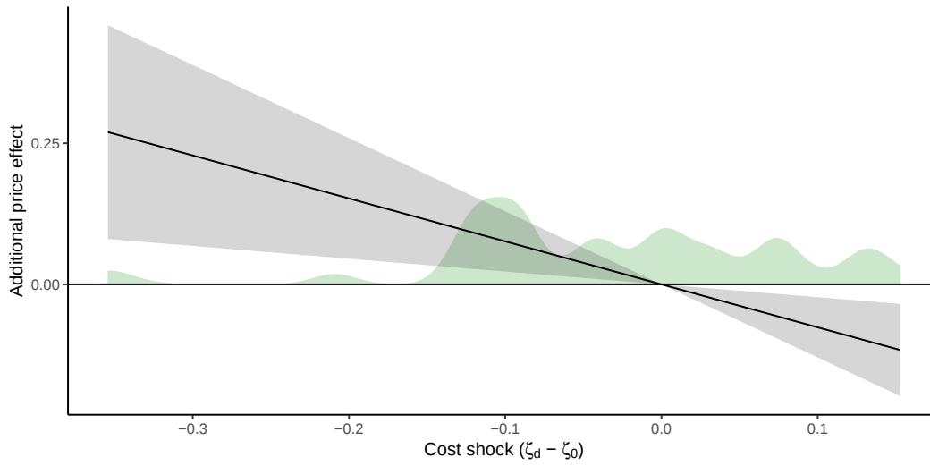
Figure A47: Effect heterogeneity by implied cost shocks \zeta_d - \zeta_0 on home prices
