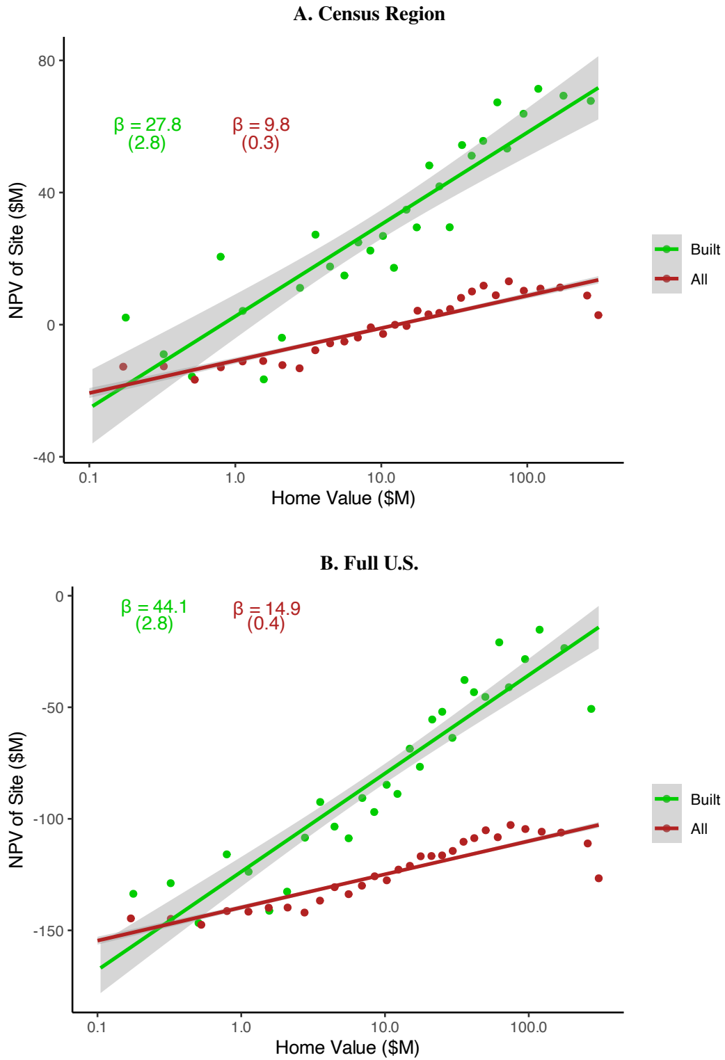
Figure A3: Profitability of selected sites and home values: Different residualizations
