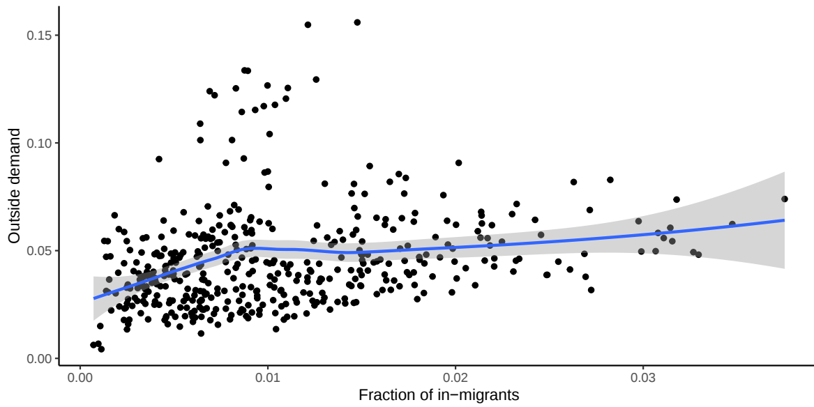
Figure A12: Relationship between outside demand and the ex-ante fraction of in-migrants
