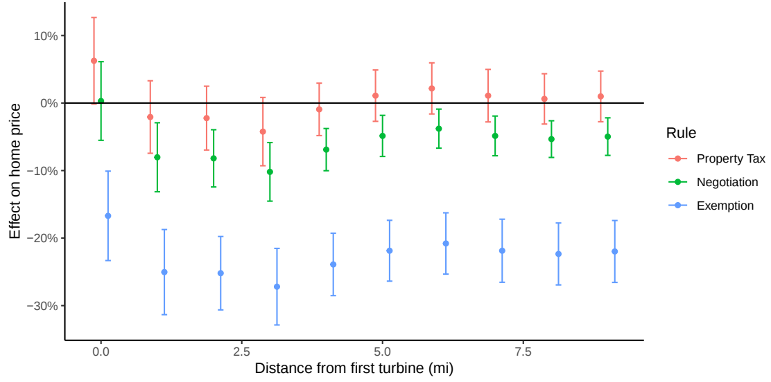
Figure A25: Effects of wind farm entry on property values by distance and tax rule
