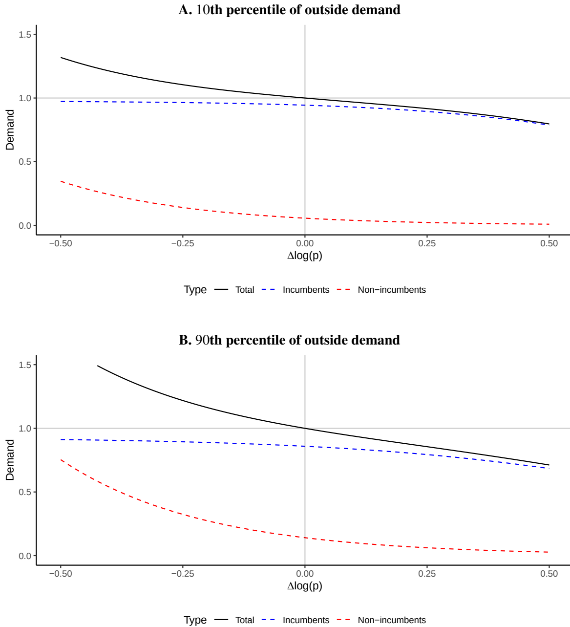
Figure A13: Demand curves of eventually treated locations
