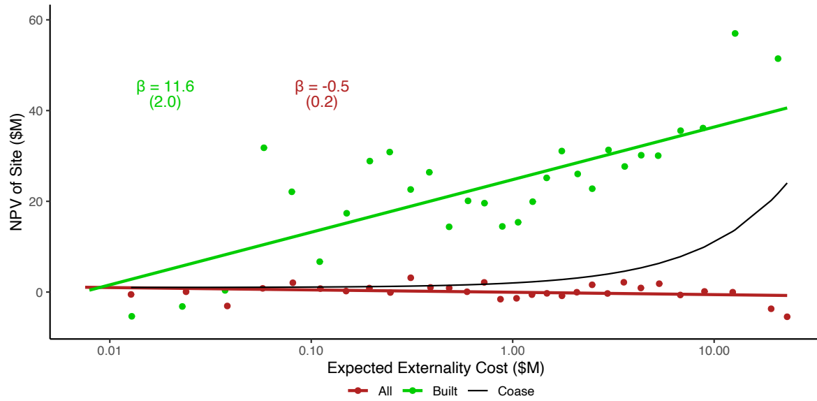
Figure A7: Profitability of selected sites and expected externality
