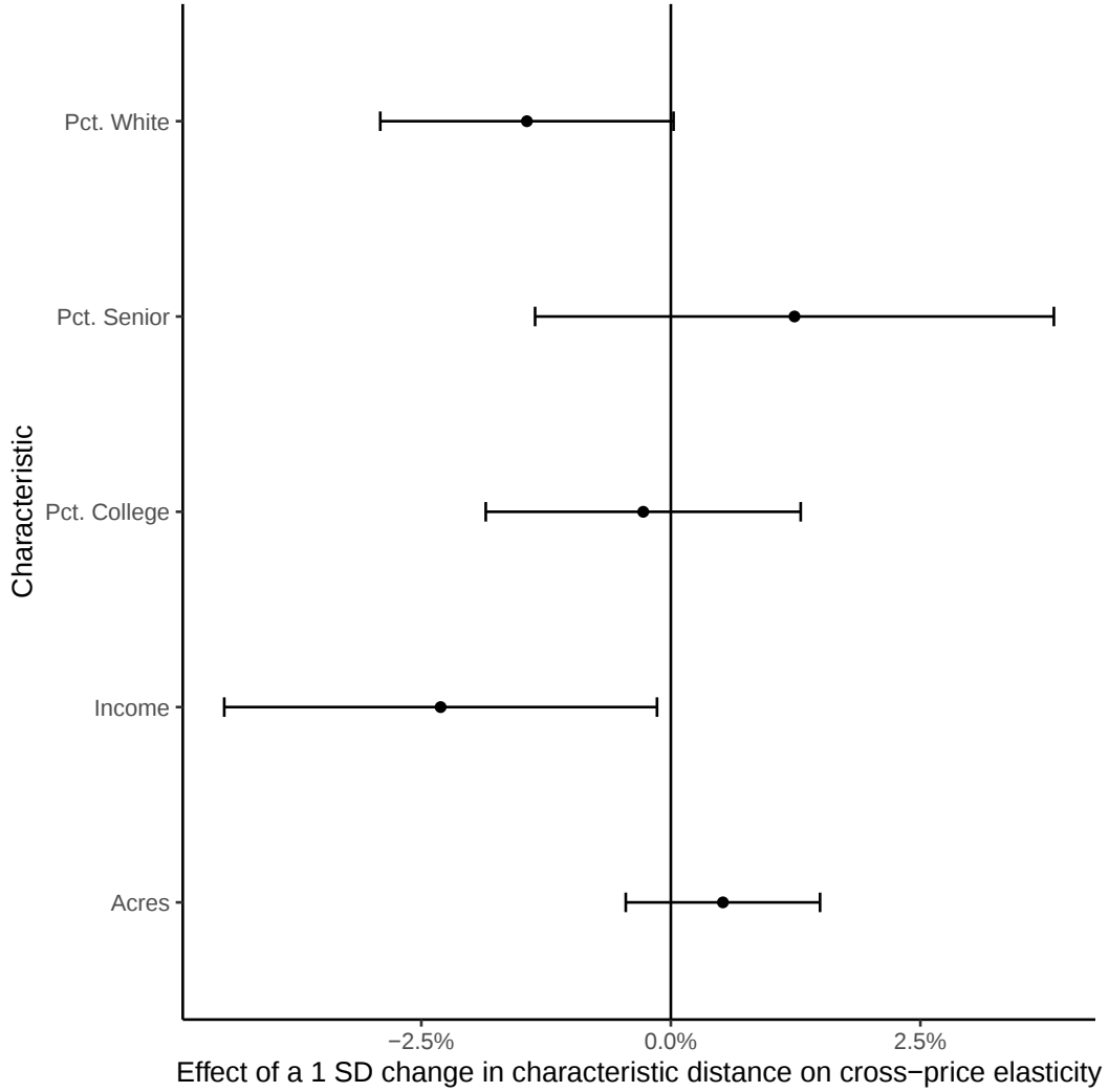
Figure A45: The effect of a 1 SD increase in characteristic distance on cross-price elasticity
