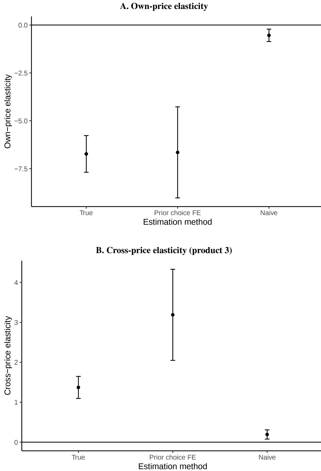
Figure A43: True price elasticities vs. estimates
