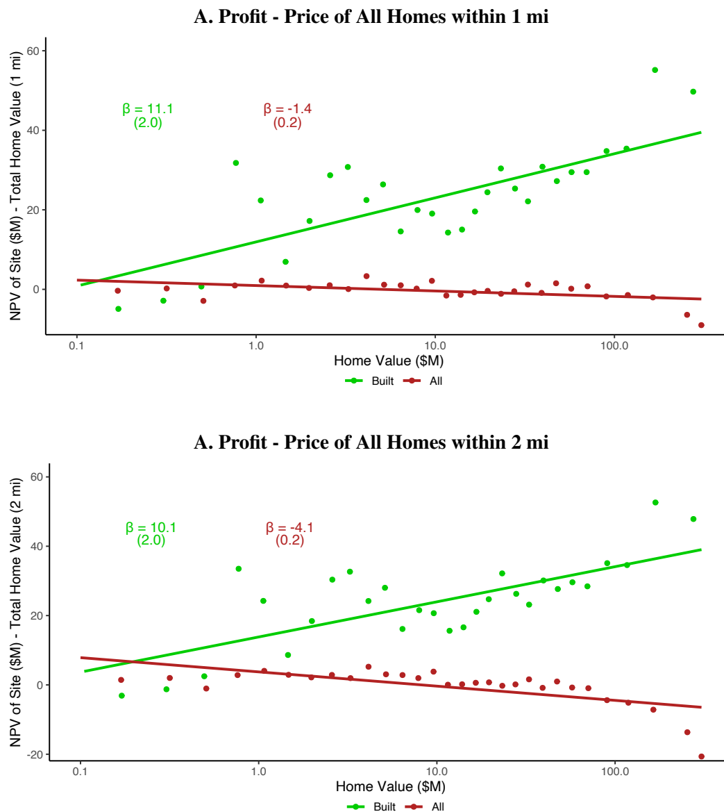
Figure A2: Profitability of selected sites and home values: Different profit calculations
