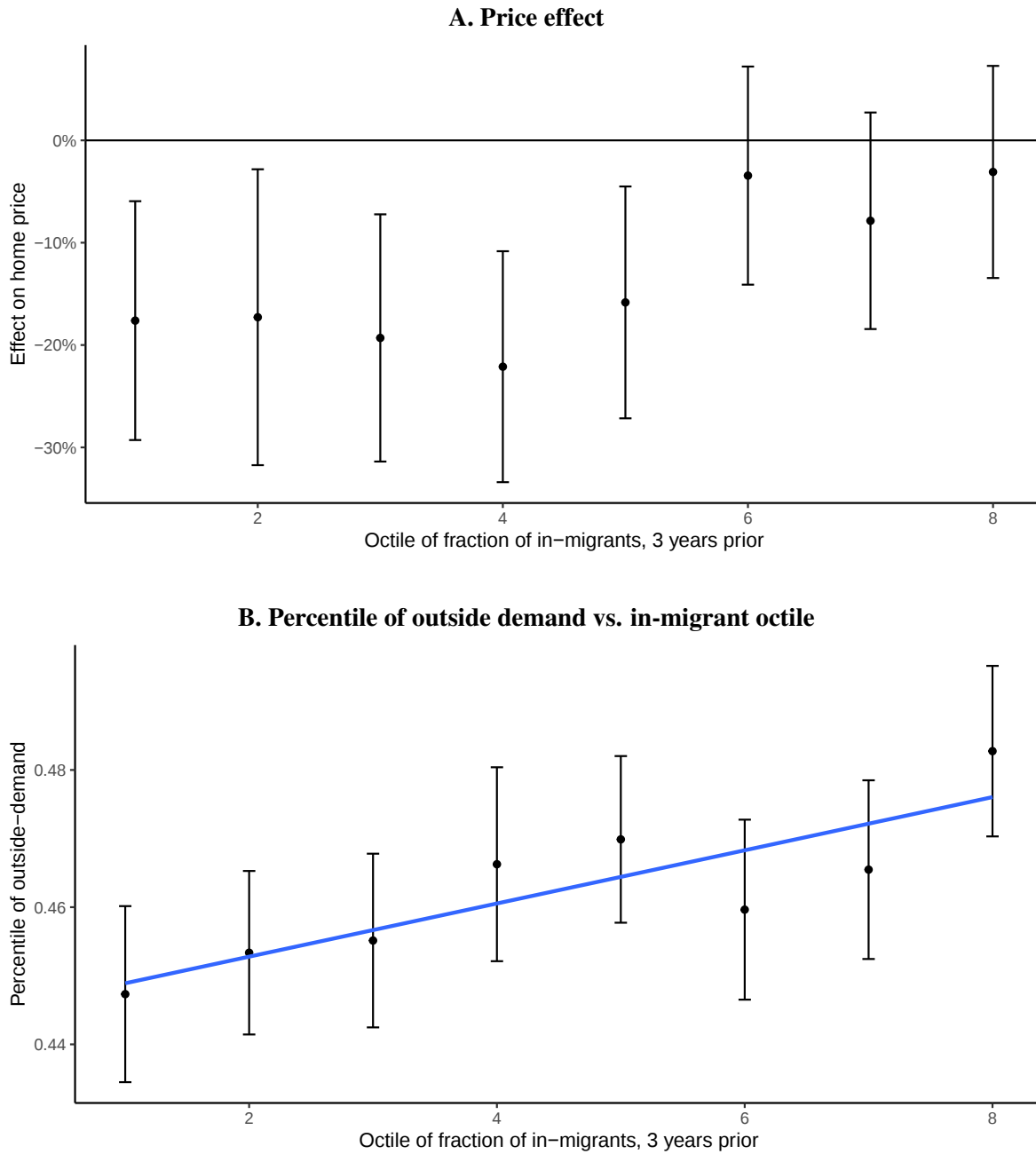
Figure A15: Effect of wind farms on price by pre-period in-migrants
