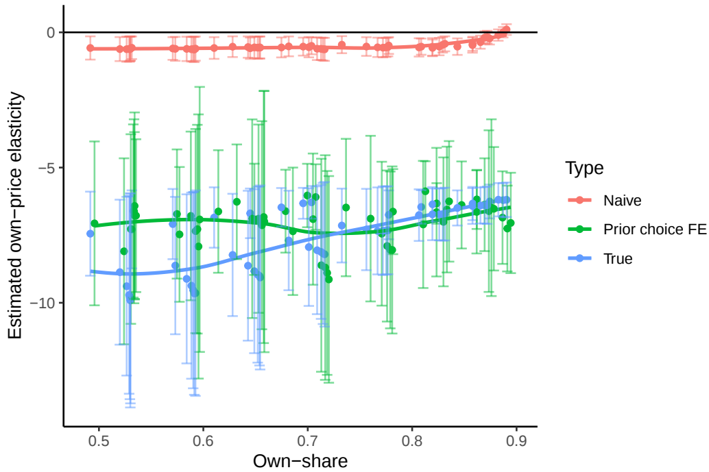
Figure A44: Simulated elasticities and estimates
