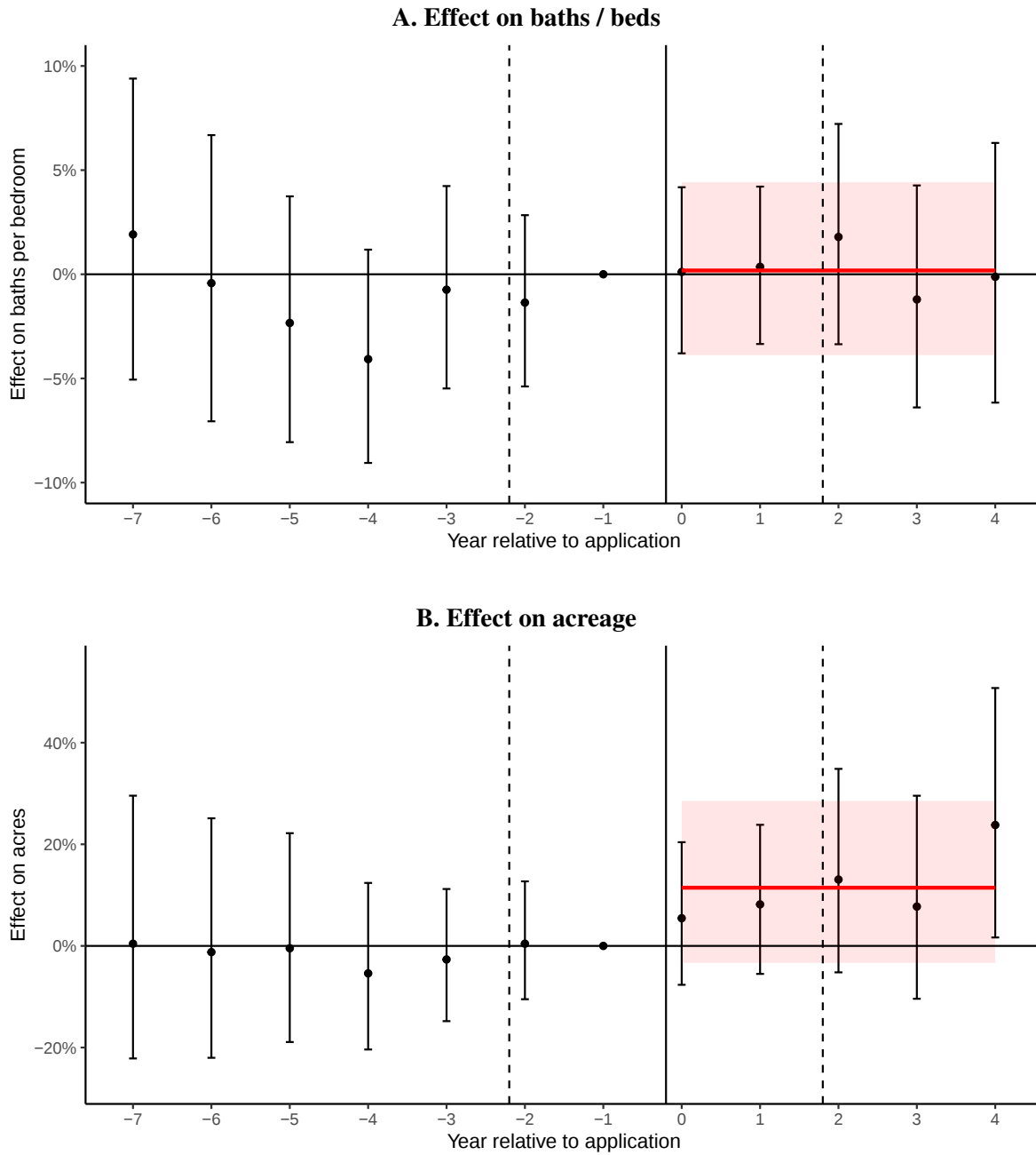
Figure A5: Effects of wind farm entry on transacted home characteristics within 5 miles
