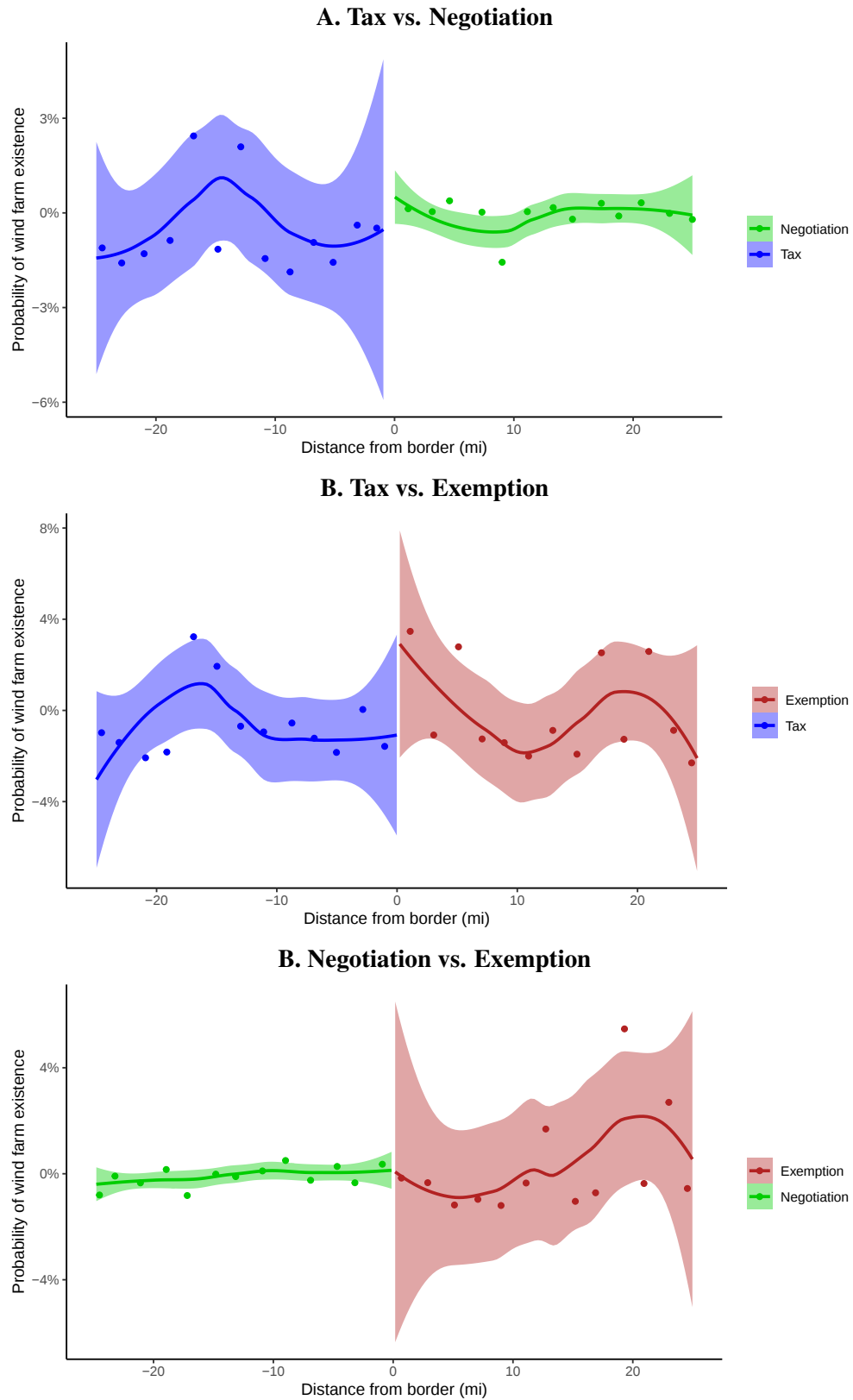
Figure A19: Border RDD effects of tax rule on existence ( \leq 1 house within 5 mi)
