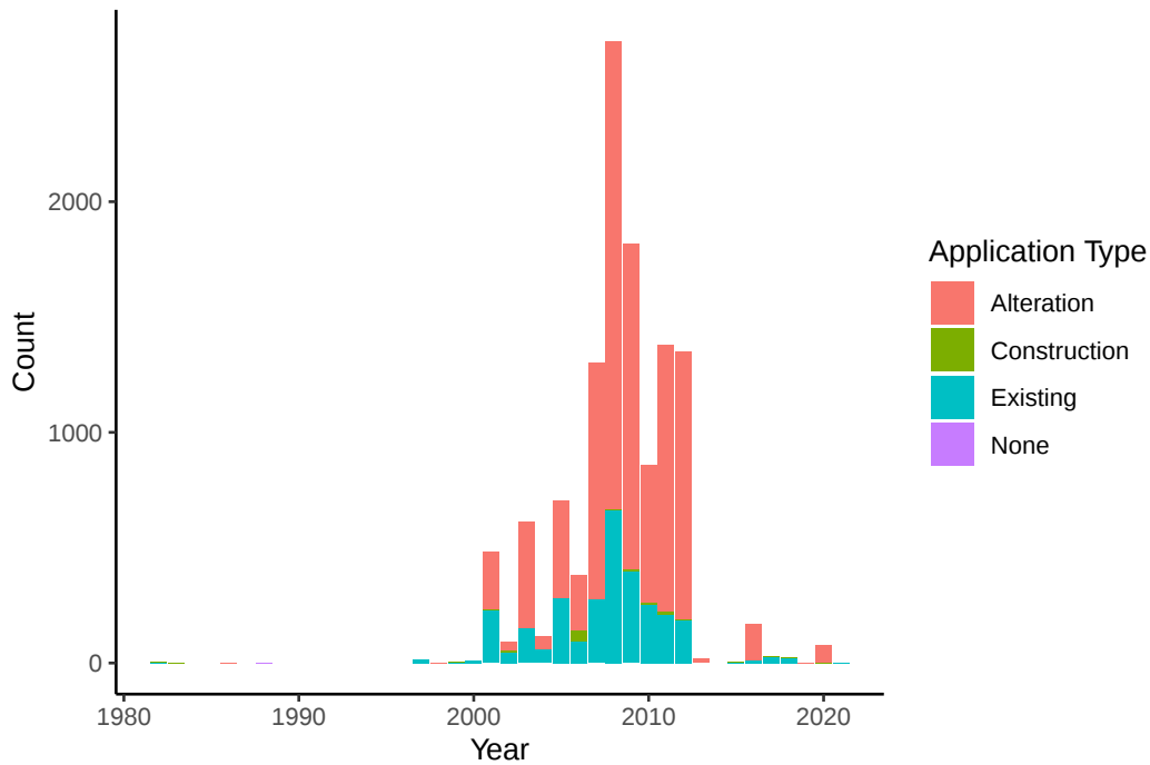
Figure A30: Stated reasons for applications after project year
