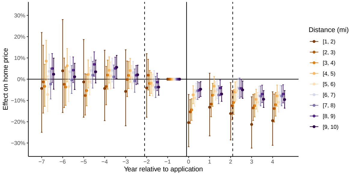
Figure 2: Effects of wind farm entry on property values within 10 miles
