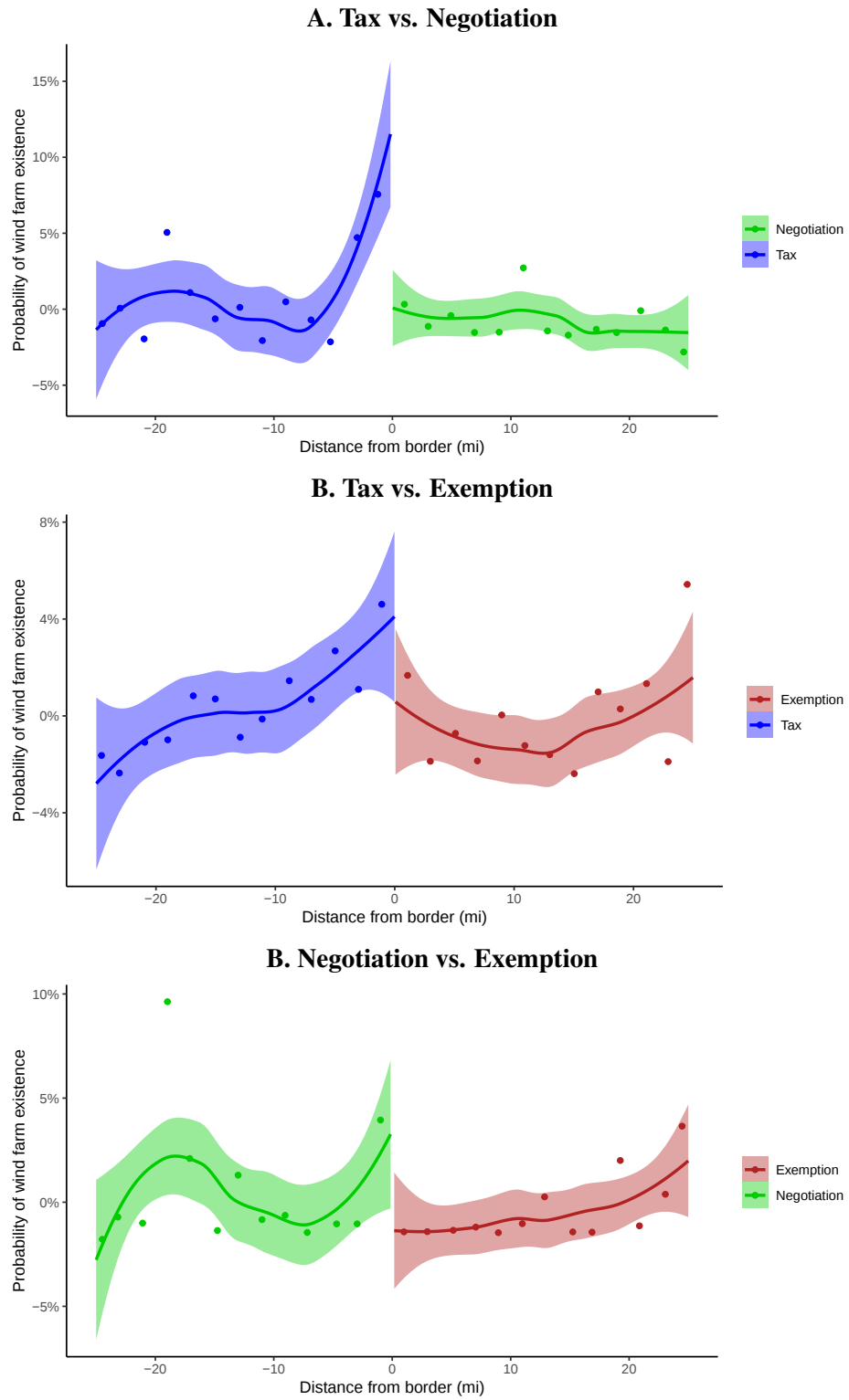
Figure 6: Border RDD effects of tax rule on existence
