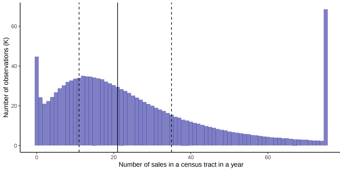
Figure A9: Distribution of number of homes sold in each census tract per year
