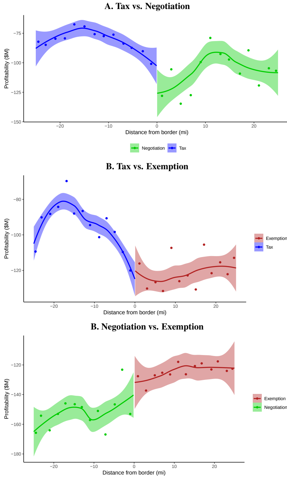
Figure A20: Balance of profit at borders
