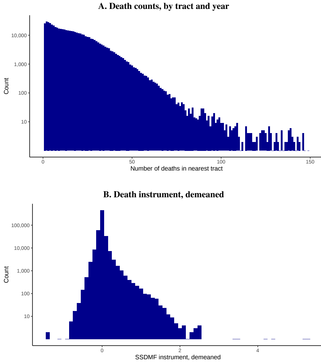
Figure A10: Histogram of death instrument values
