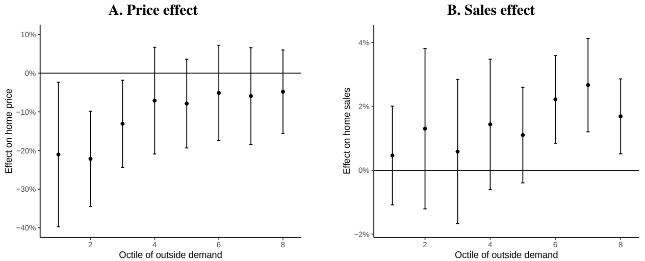
Figure 3: Effect of wind farms on price and sales volume by outside demand
