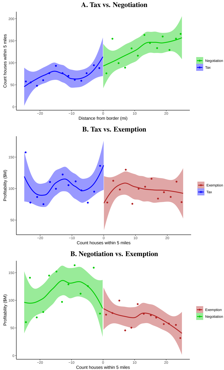
Figure A21: Balance of the number of houses within 5 miles at borders
