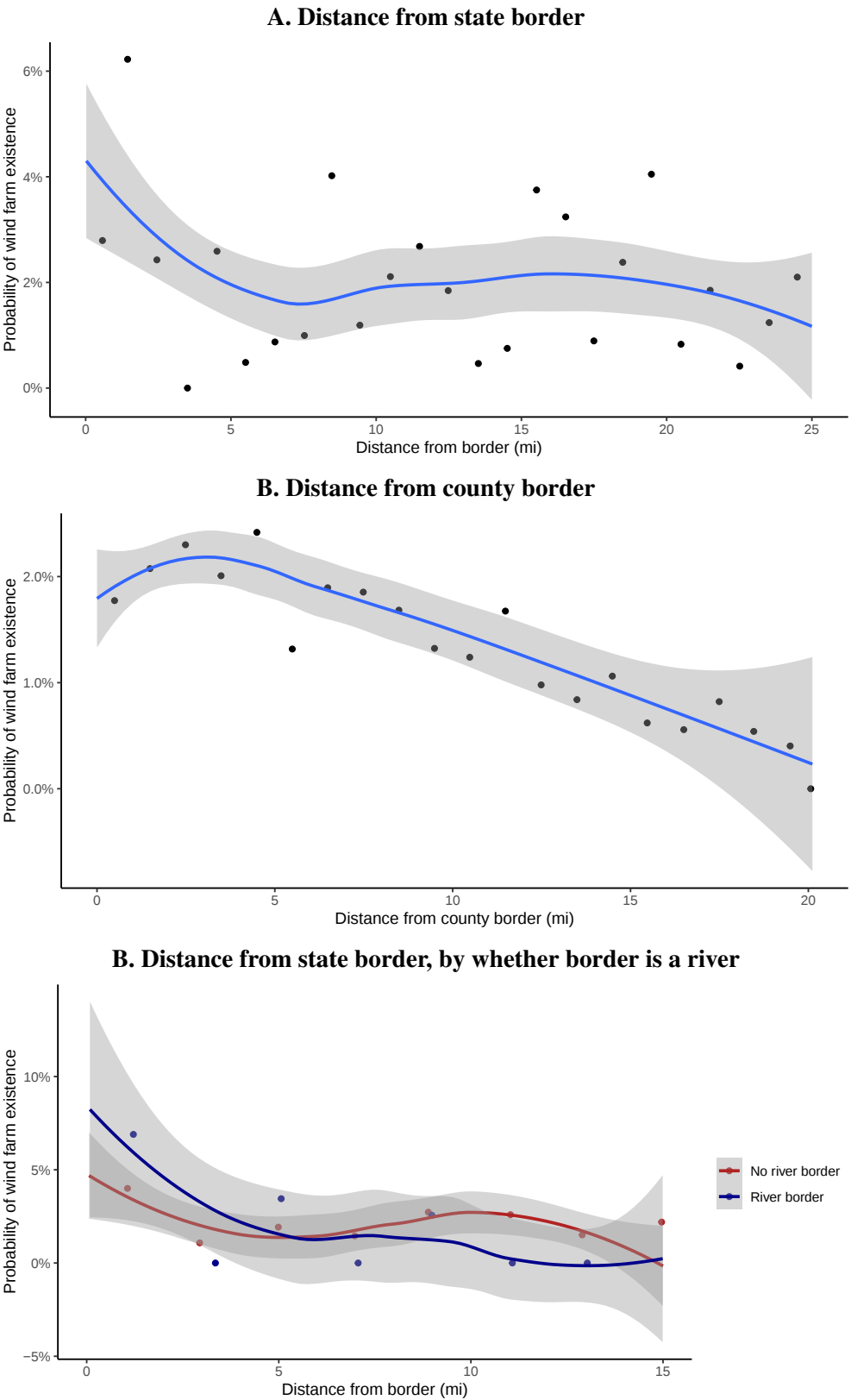
Figure A22: Relationship of likelihood of construction to distance from border
