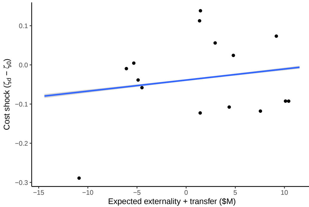
Figure A48: Bin-scatter of expected net local cost and the posterior of \zeta_d - \zeta_0
