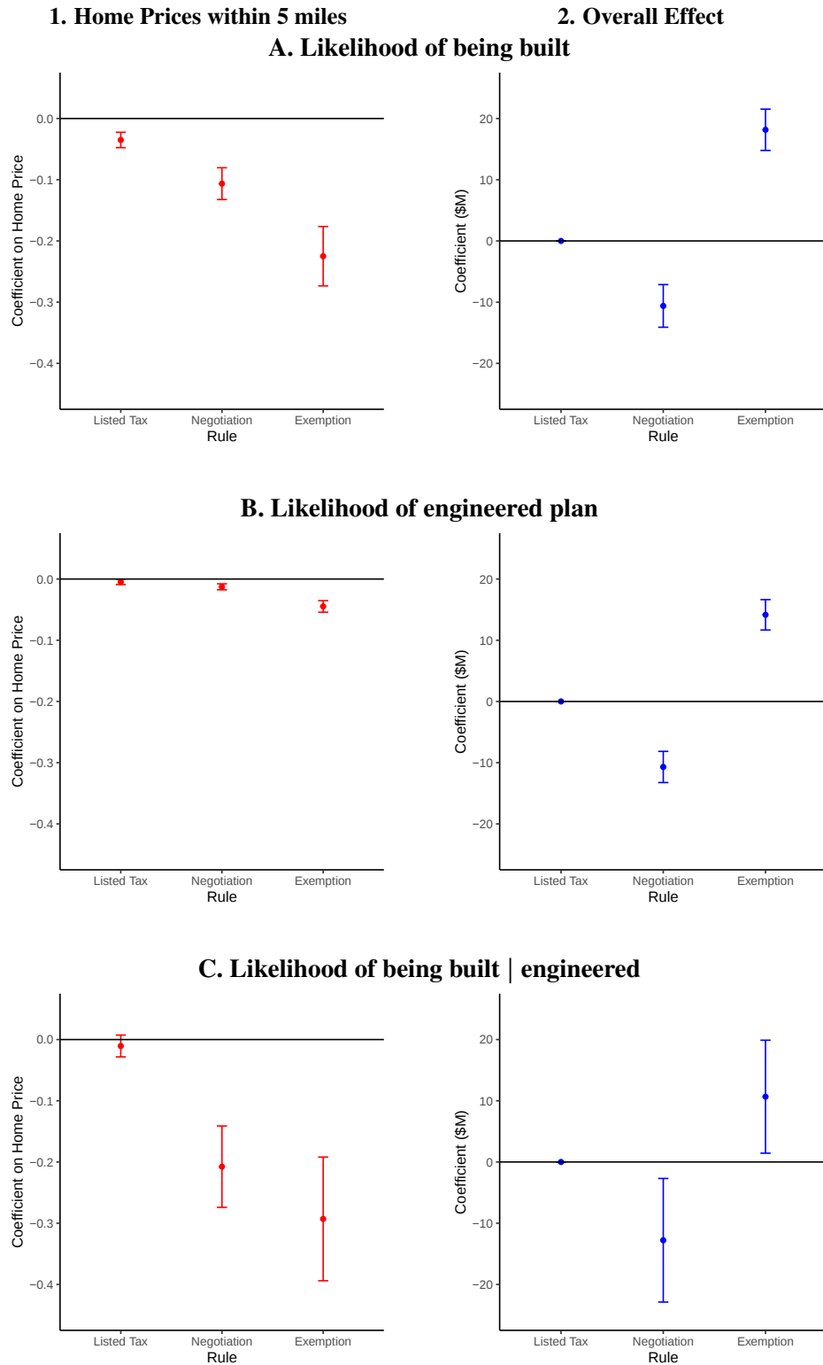
Figure A26: Relationship of entry margins & key covariates across regimes
