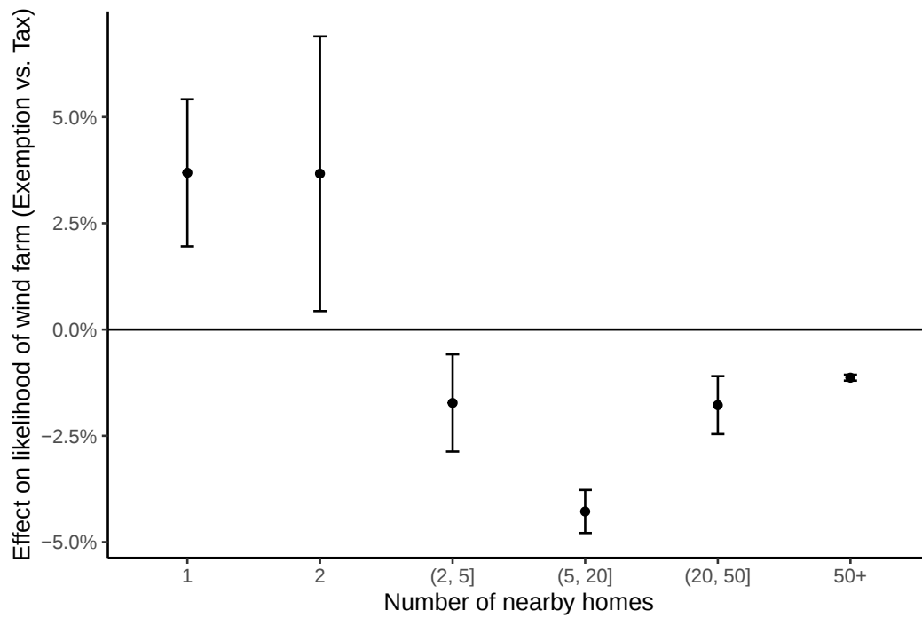
Figure A23: Border effect of exemption vs. tax by number of nearby homes
