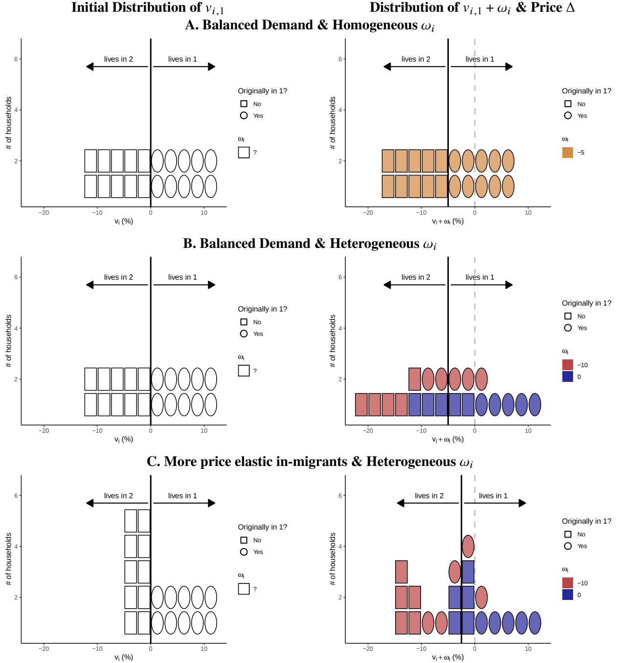
Figure A41: Illustration of how the shape of demand curves affect price and re-sorting
