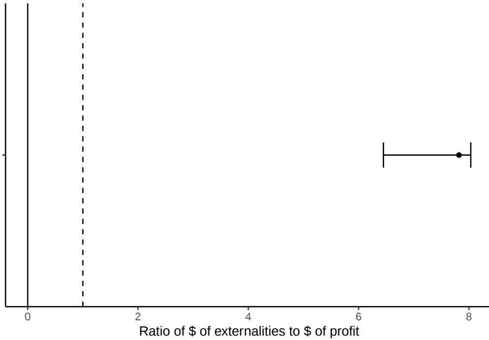
Figure A38: Trade-off between profit and externality
