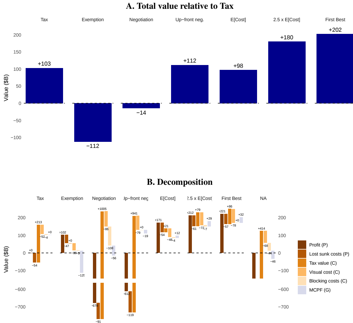
Figure 8: Social welfare under alternative market designs
