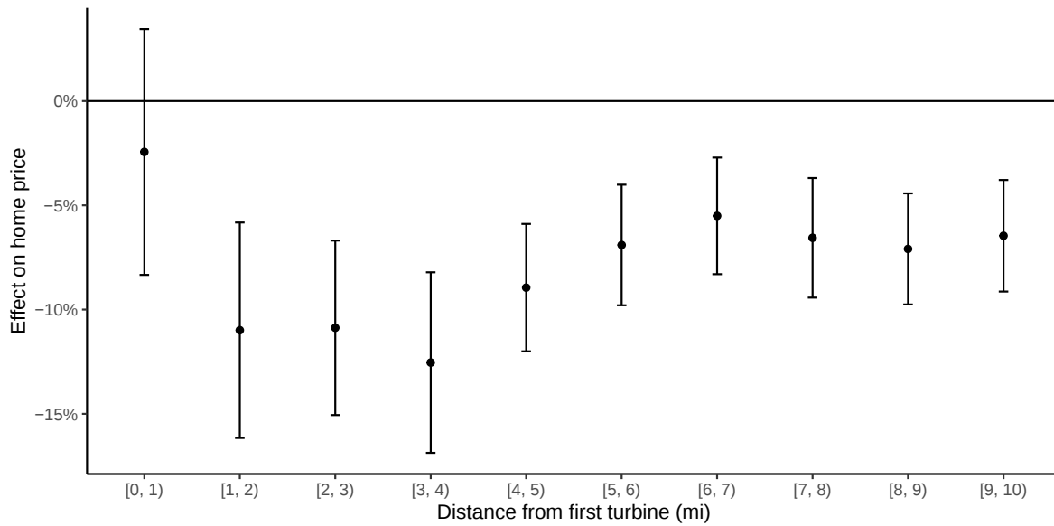
Figure A4: Price effects by distance from turbine
