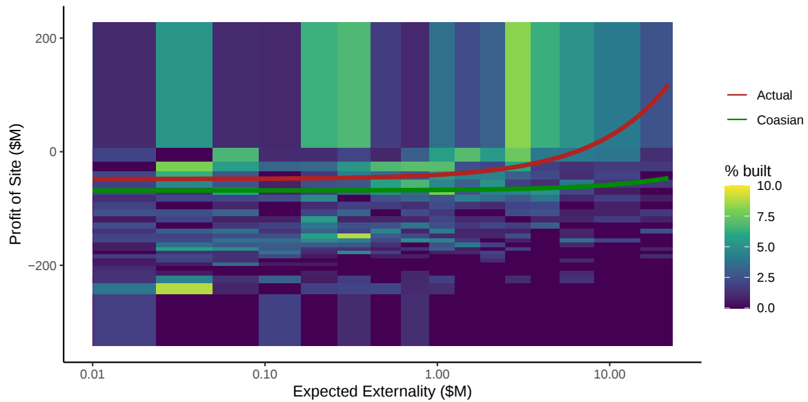
Figure A8: Heat map of probability of construction by profit and externality
