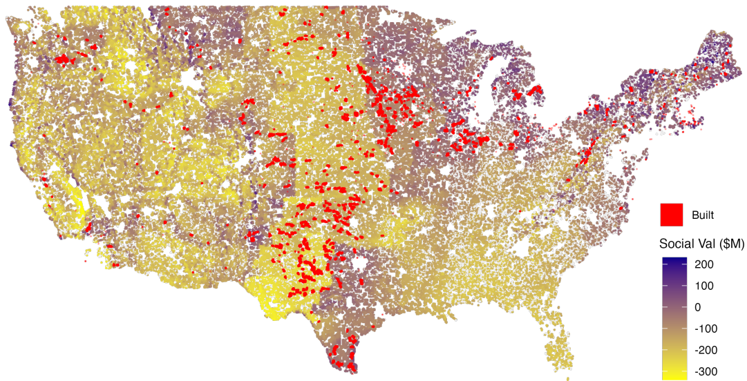
Figure A16: Net social value and constructed wind farms
