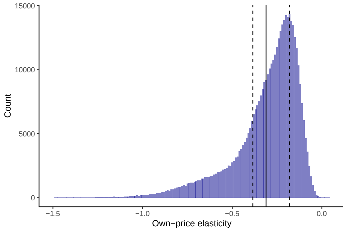
Figure A11: Histogram of estimated own-price elasticities of all census tracts
