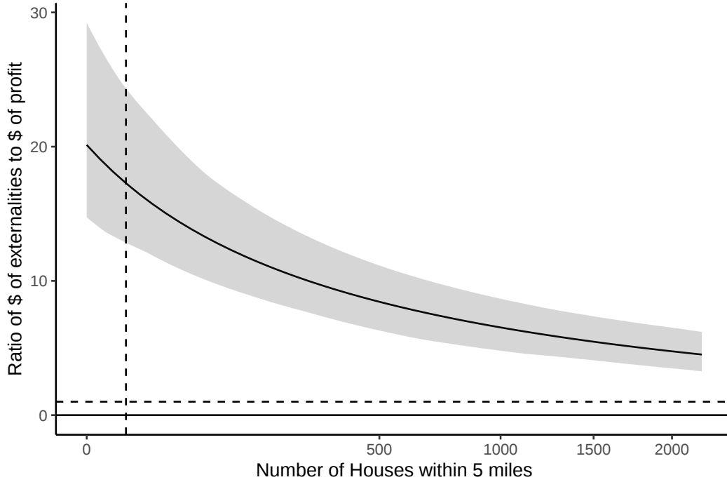
Figure A39: Trade-off between profit and externality: data-driven variance of the unobservable
