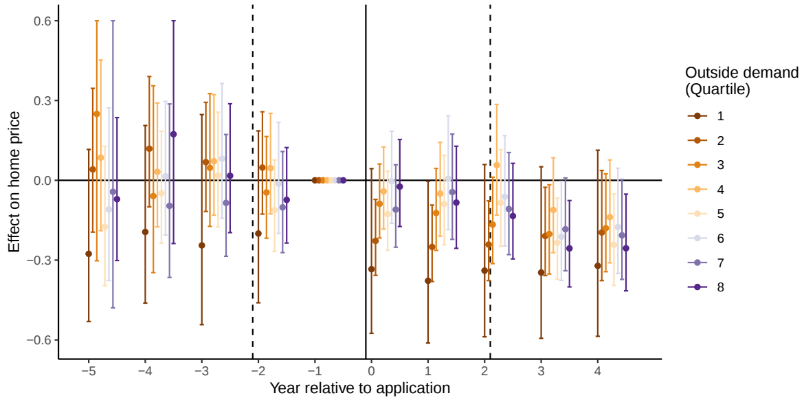
Figure A14: Effects of wind farm entry on home values by outside demand
