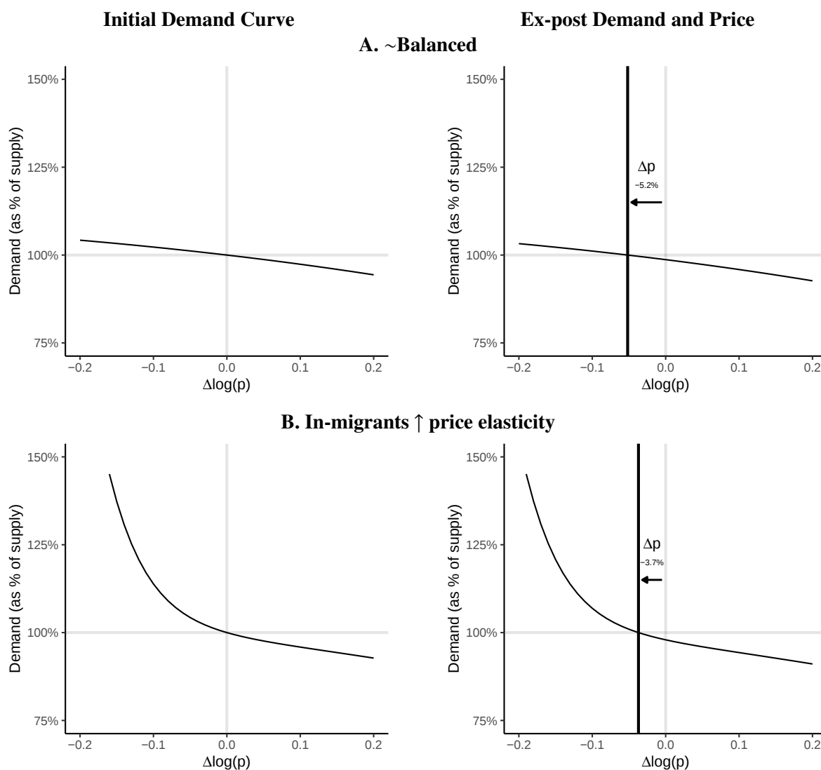
Figure A40: Relating the shape of demand curves and equilibrium price changes
